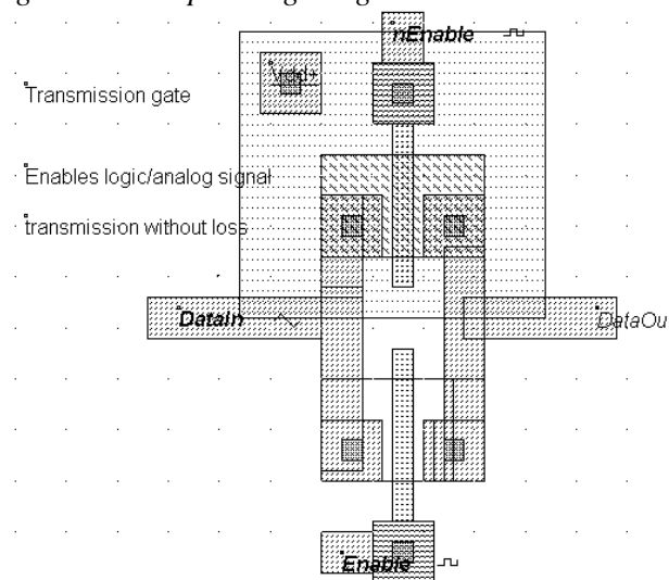
Fig. 3-23. Layout of the transmission gate (TGATE.MSK)
