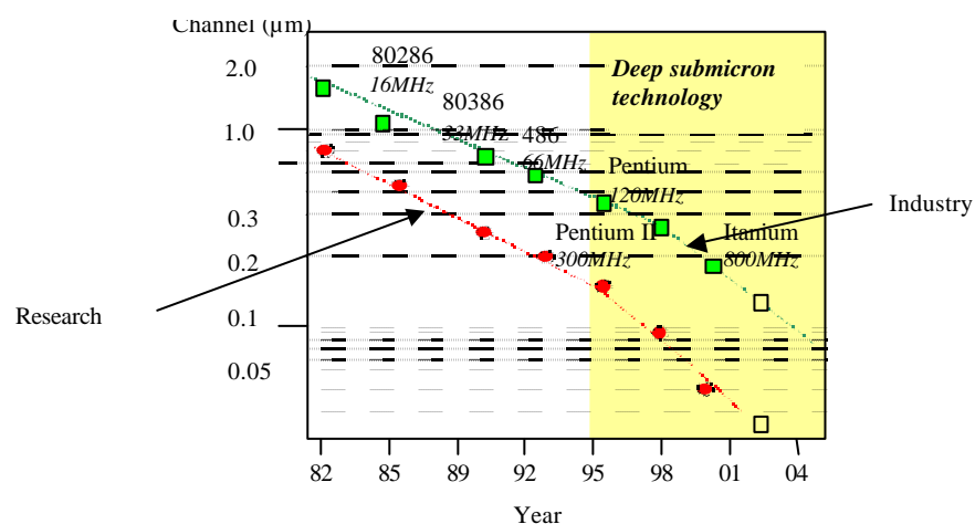
Fig. 2-3: Evolution of lithography
