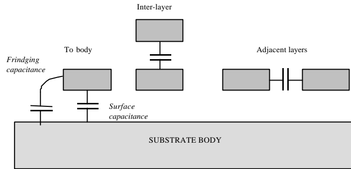
Figure 12-2: Capacitances
