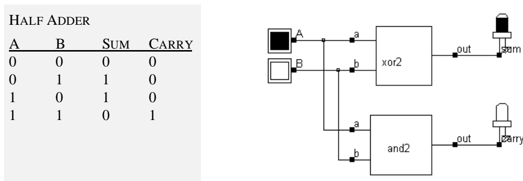
Fig. 6-1. Truth table and schematic diagram of the half-adder gate (HADD.MSK).
