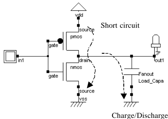
Fig. 4-4: Short circuit current in CMOS inverters
