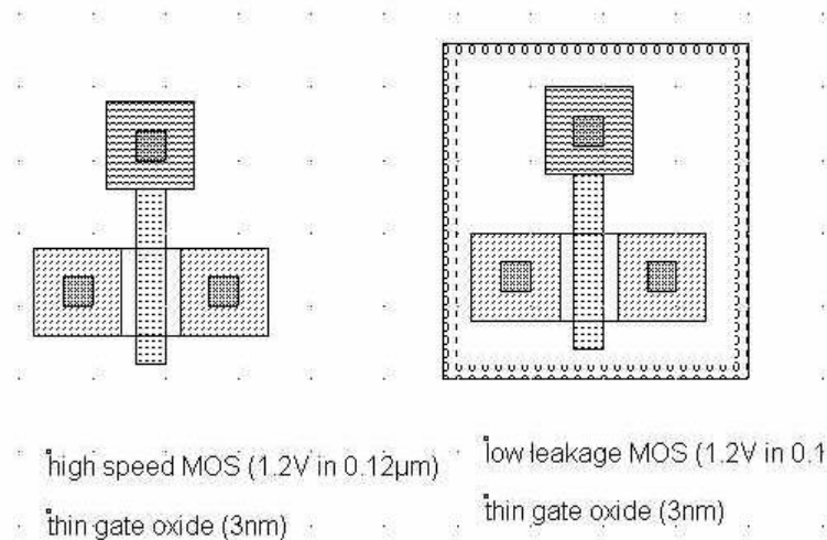
Fig. 3-15: High speed and Low leakage MOS layout. The only difference is the option layer configured for the low leakage option
