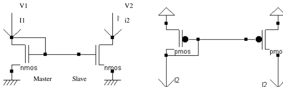
Figure 8-5: Current mirror principles in nMOS and pMOS versions
