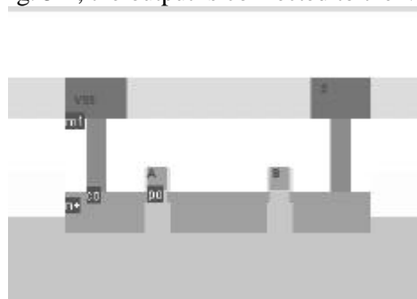
Fig. 5-4. The nMOS devices in serial in the NAND gate
