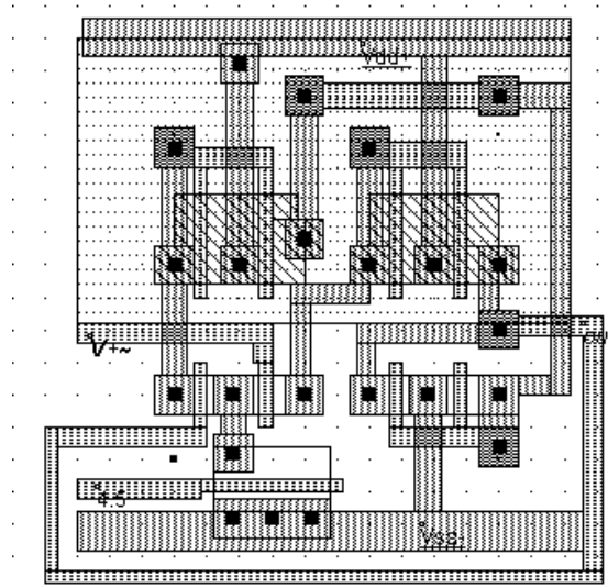
Fig. 8-14. Design of the analog amplifier (AMPLI2.MSK).
